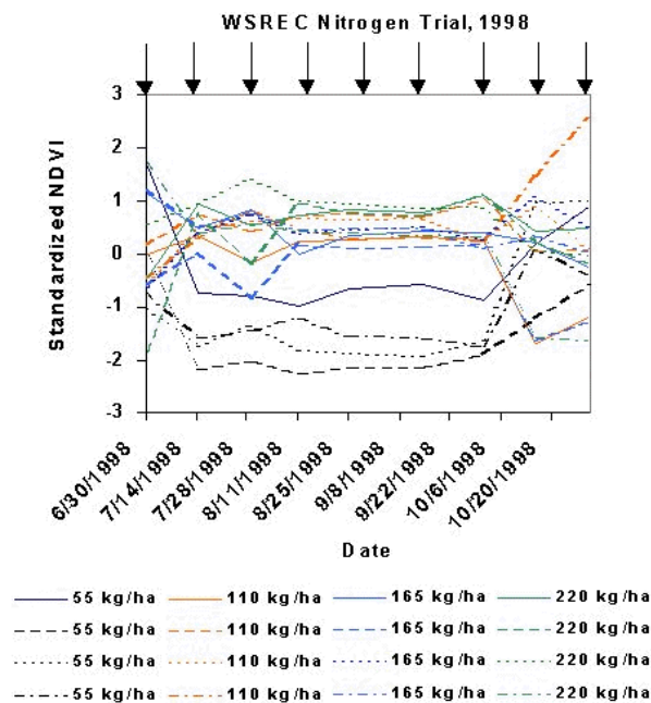
Fig. 4. Standardized normalized difference vegetation index (NDVI) values vs. date for each of the individual plots in the N experiment conducted at the Univ. of California West Side Res. and Ext. Ctr. (WSREC) in 1998. The treatments are total N rates.
