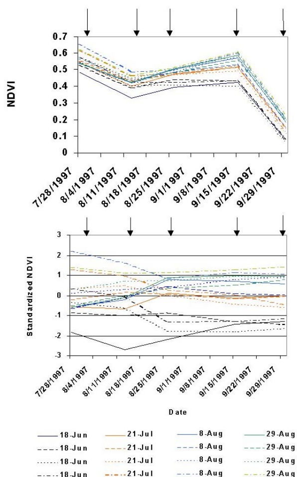
Fig. 1. (a) Average plot--normalized difference vegetation index (NDVI) vs. date for each of the individual plots in the irrigation experiment conducted at the Univ. of California West Side Res. and Ext. Ctr. in 1997. The treatments, distinguished by color, are date of last irrigation. The individual plots are distinguished by form of curve. Arrows indicate dates on which photographs were taken. Note that all curves tend to move up and down together. (b) Standardized values of the same data shown in Fig. 1a. The data were standardized by subtracting the daily mean and dividing by the daily standard deviation. The curves tend to sort themselves out after 25 Aug. and remain in the same order.
